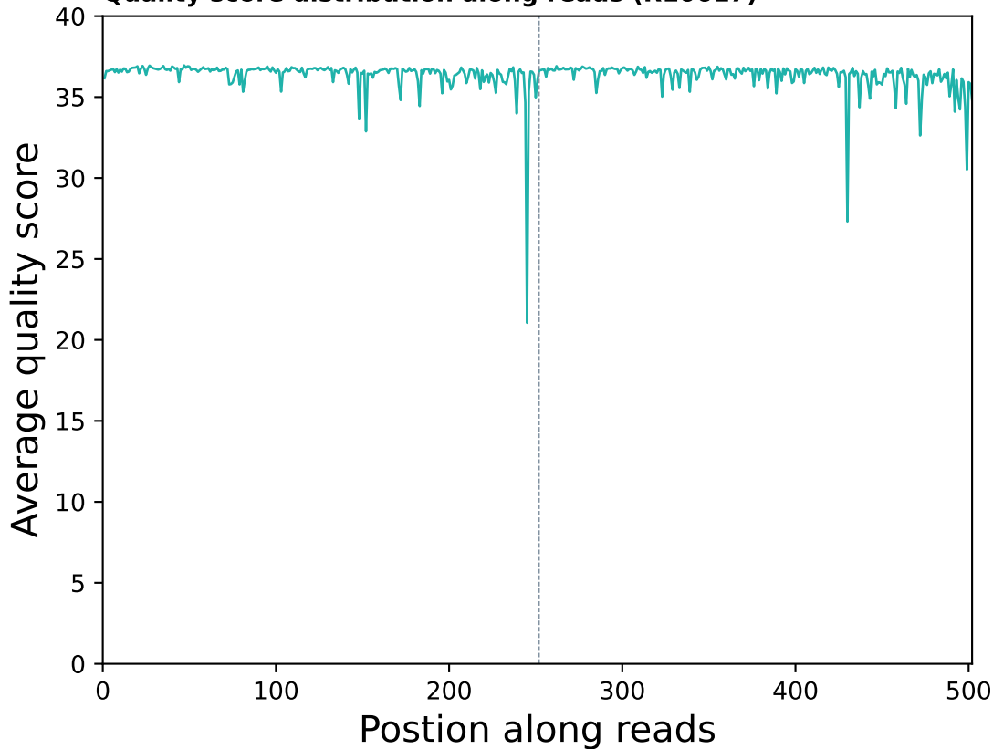
Quality score distribution along reads (R10617)
